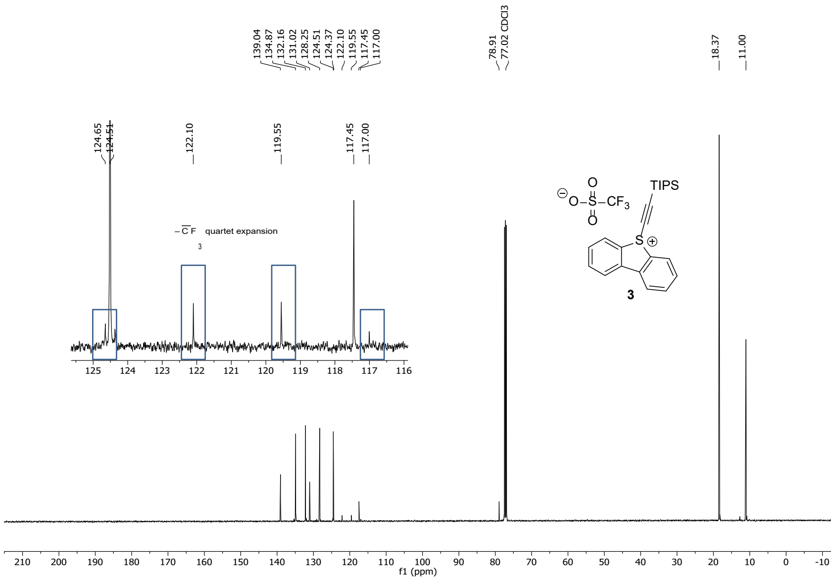
^{13}\text{C} NMR spectrum of 5-(triisopropylalkynyl)-dibenzo[ b,d ]thiophenium triflate 3 in CDCl 3 at 126 MHz
